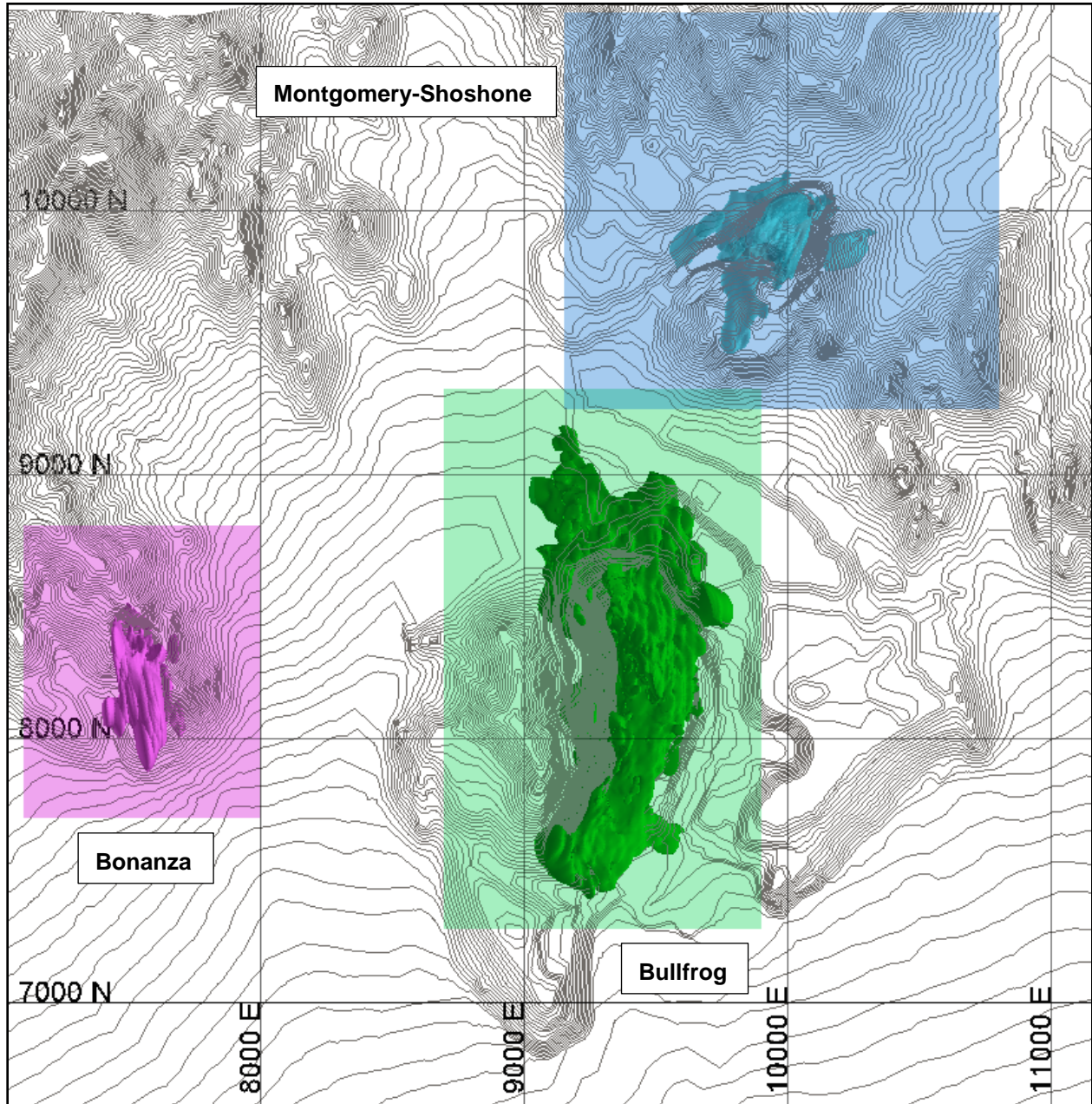
Figure 14-2: Grade Shell (DOMAIN) Triangulations
