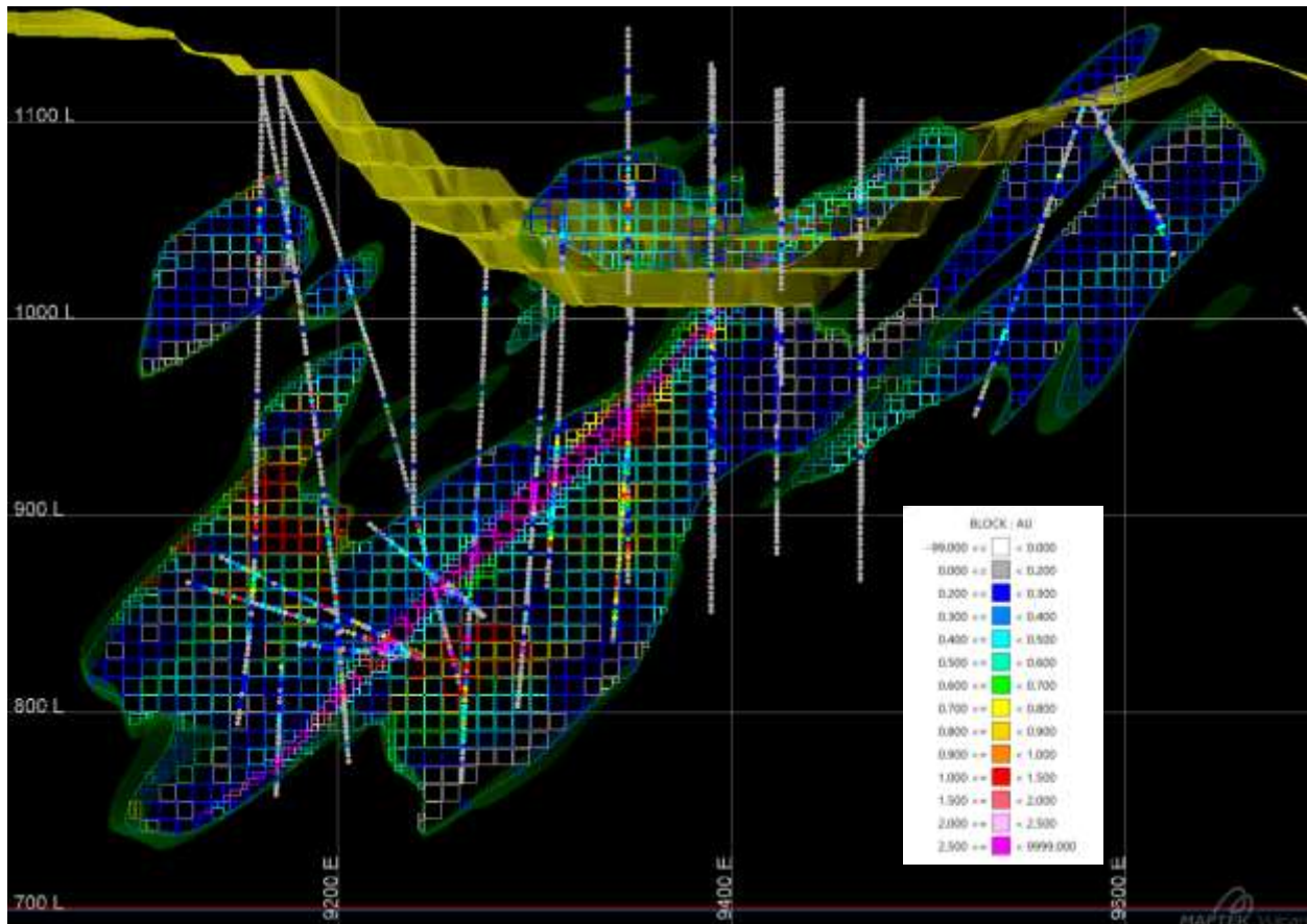
Figure 14-8: Bullfrog 8620N Cross-Section Showing Gold Blocks and Composites
